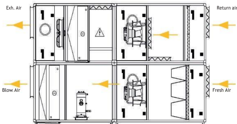
Free-cooling Mode
